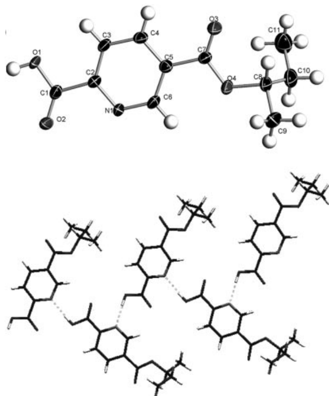
Figure 1. Top: XSEHELL plot of 2b (50% probability level). Bottom: Hydrogen bonding network for 2b (Mercury, vers. 1.1).
