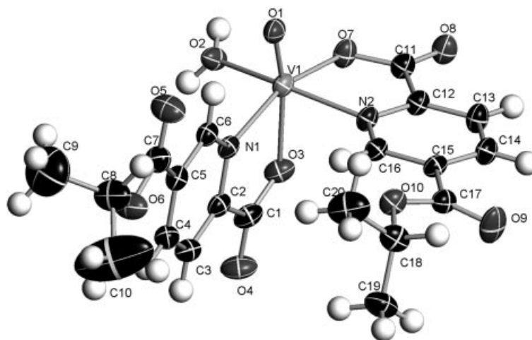
Figure 4. XSHELL plot of 4a (50% probability level). Only one of the two independent molecules, containing one of the i Pr substituents in a disordered state, is shown. Water of crystallization omitted. Selected bonding parameters: V1–O1 1.5989(14), V1–O2 2.0175(14), V1–O3 1.1290(15), V1–O7 1.9890(15), V1–N1 2.1503(17), V1–N2 2.1072(16) Å; O1–V1–O3 164.55(7), O2–V1–N2 164.62(7), O7–V1–N1 161.62(6)°.
