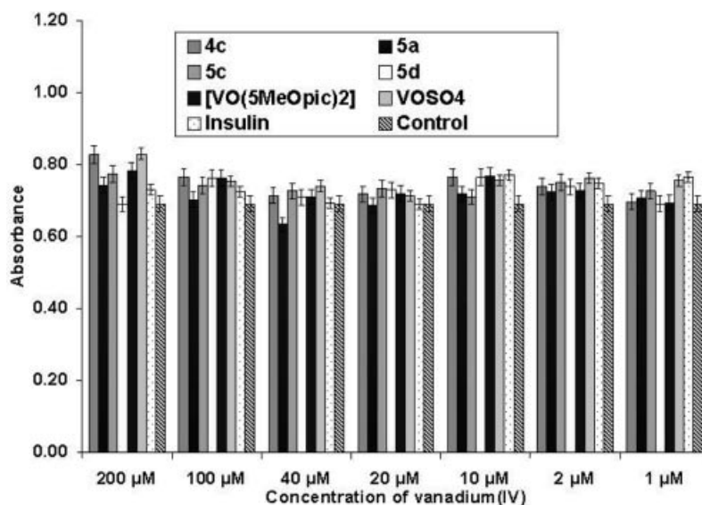
Figure 5. Glucose uptake stimulated by the vanadium picolates 4c , 5a , 5c and 5d after 60 min. The absorbance, shown relative to a control group, reflects the efficacy of the compounds. The diagram also shows the data for [\text{VO}(\text{5MeOpic})_2] , \text{VOSO}_4 , and a group of cells where insulin was added instead of vanadium.
