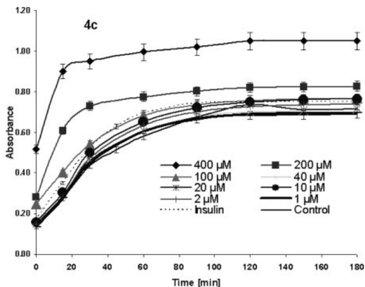
Figure 7. Glucose uptake stimulated by the galactosyl derivative 4c as a function of time over a wide concentration range. Data are not corrected for background.
