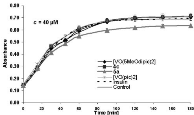
Figure 6. Glucose uptake stimulated by 4c and 5a ( c = 40 \mu\text{M} ) presented as a function of time. This diagram also includes the results for [\text{VO}(\text{pic})_2] , [\text{VO}(\text{5MeOdic})_2] and insulin. Data are not corrected for background.
