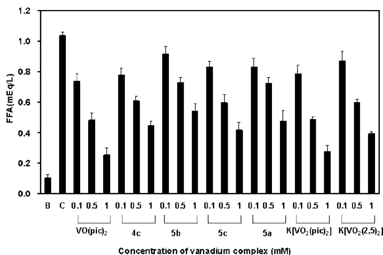
Figure 8. Inhibitory effects of vanadium complexes on FFA-release from rat adipocytes treated with epinephrine. Data are expressed as the means \pm SDs for three experiments. B: adipocytes treated with insulin. C: adipocytes pre-incubated with saline for 30 min before treatment with 10 \mu M epinephrine for 3 h.
