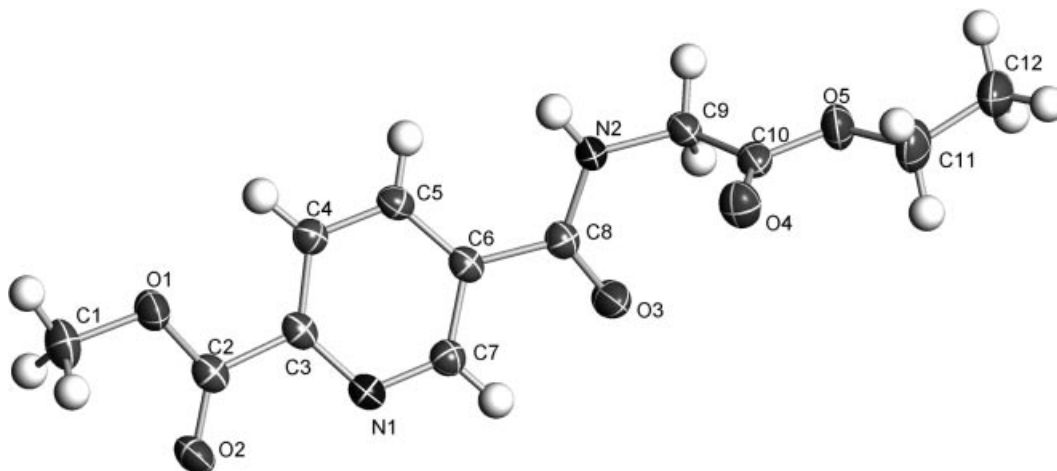
Figure 2. XSEHELL plot of 3a (50% probability level).
