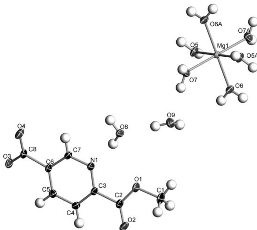
Figure 3. XSHELL plot of [\text{Mg}(\text{H}_2\text{O})_6](1\text{H}_{-1})_2 \cdot 4\text{H}_2\text{O} (50% probability level). Only one of the anions 1\text{H}_{-1} and two of the waters of crystallization are shown.
